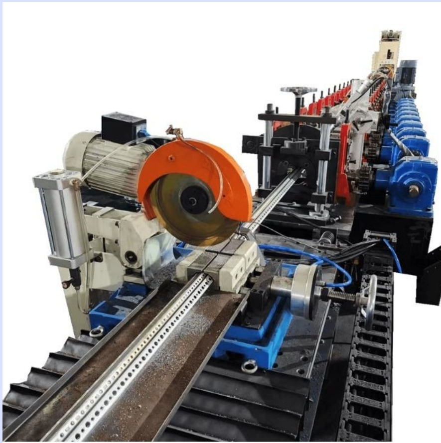
Gearbox Driven Steel Storage Rack Roll Forming Machine With Advanced Punching Capability
